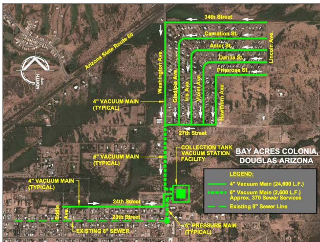
Figure 2.7: Vacuum Collection System
